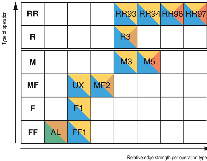
Chipbreaker chart for positive basic shape inserts
