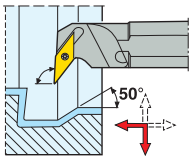
SVUBR/L KAPR = 93,0 °
