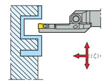
CFOR/L KAPR = 90,0 °
