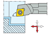
SCLCR/L KAPR = 95,0 °
