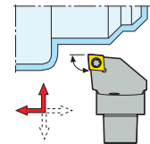
C-SCLCR/L KAPR = 95,0 °
