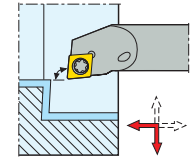
C-SCLCR/L KAPRI = 95,0 °
