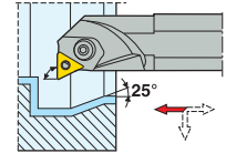
PTFNR/L A32, A40, A50 KAPR = 90,0 °
