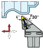
C.-DDJNR/L...JETI KAPR = 93,0°
