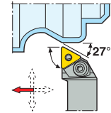
PTGNR/L, -..A KAPR = 90,0°
