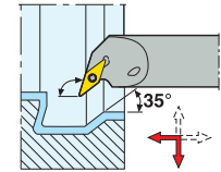
C.-SVQBR/L KAPR = 107,5°
