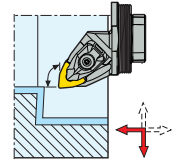
GL..-DWLNR/L KAPR = 95,0 °
