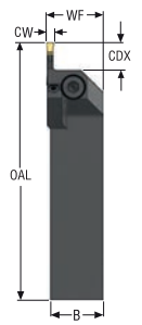
CFIR/L2020...JETI
