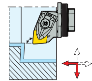
GL..-DCLNR/L KAPR = 95,0 °
