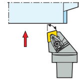
C-DCKNR/L, -M KAPR = 75,0 °
