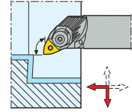
C.-PWLNR/L KAPR = 95,0 °
