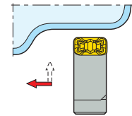
CT-PLFNR/L KAPR = 90,0 °
