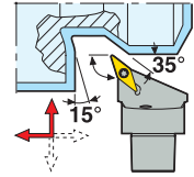
C.-SVHBR/L KAPR = 107,5°
