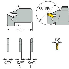
HSS-blade 150.10A-15
