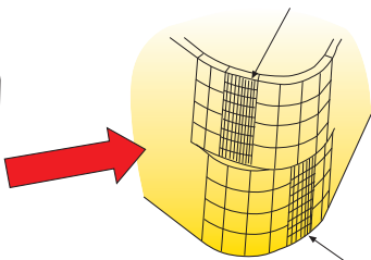
Wiper segment
