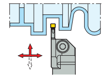
CFMR/L KAPR = 90,0 °
