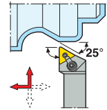
MTJNRS/LS KAPR = 93,0 °
