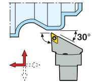
C.-SDJCR/L KAPR = 93,0 °
