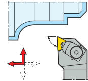
CTFNR/L KAPR = 91,0 °
