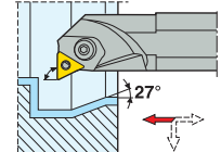
PTFNR/L A32, A40, A50 KAPR = 90,0 °
