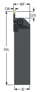
CFIR/L2525...JETI
