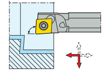
SCLCR/L..-R KAPR = 95,0 °
