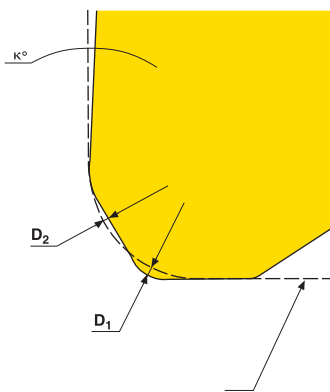
ISO-profile (Nominal nose radius)
