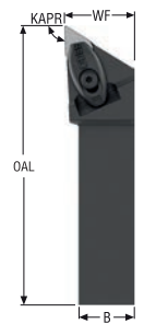
DDJNR/L1.00/1.25...JETI
