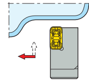
CT-PLANR/L KAPR = 90,0 °
