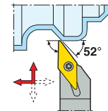
SVABR/L KAPR = 90,0 °
